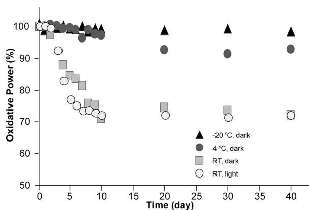
Figure 7. Oxidative power of \text{Cy}_3\text{PO}-(\text{HOO})_2\text{CMe}_2 ( 3 ) after being stored under the indicated conditions. 100% oxidative power is equivalent to 2 moles of active oxygen per mole of 3 .
