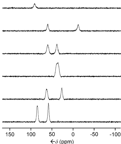
Figure 5. ^{31}\text{P} CP NMR spectra of a large single crystal of 4 at different random orientations with respect to the external magnetic field.
